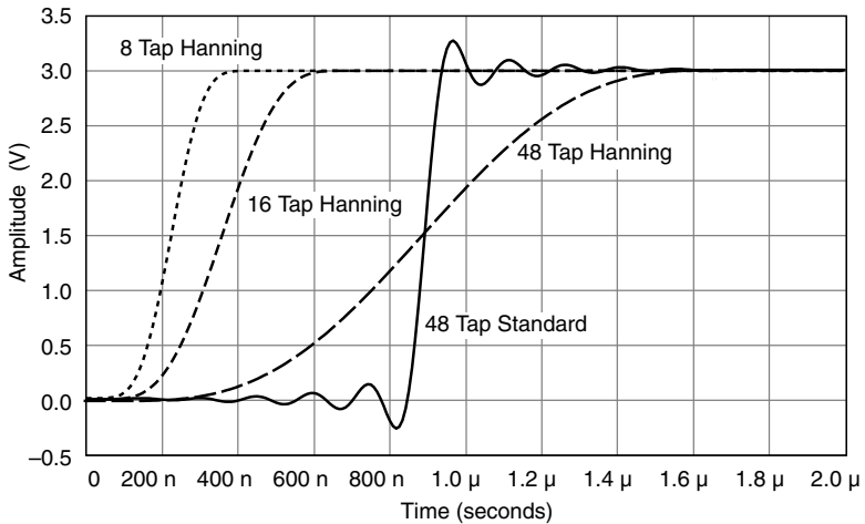
Figure 8. PXI-5922 Step Response Using Different Filter Types, Measured 17
