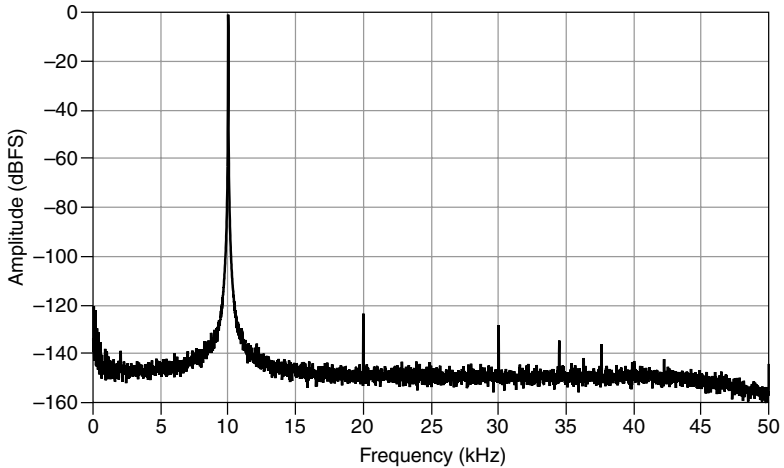
Figure 6. PXI-5922 Dynamic Performance with 10 kHz Input Signal, Measured, 1 M \Omega , 2 V pk-pk Range, 100 kS/s, Unbalanced Differential, 10,000-Point FFT with 10 Averages
